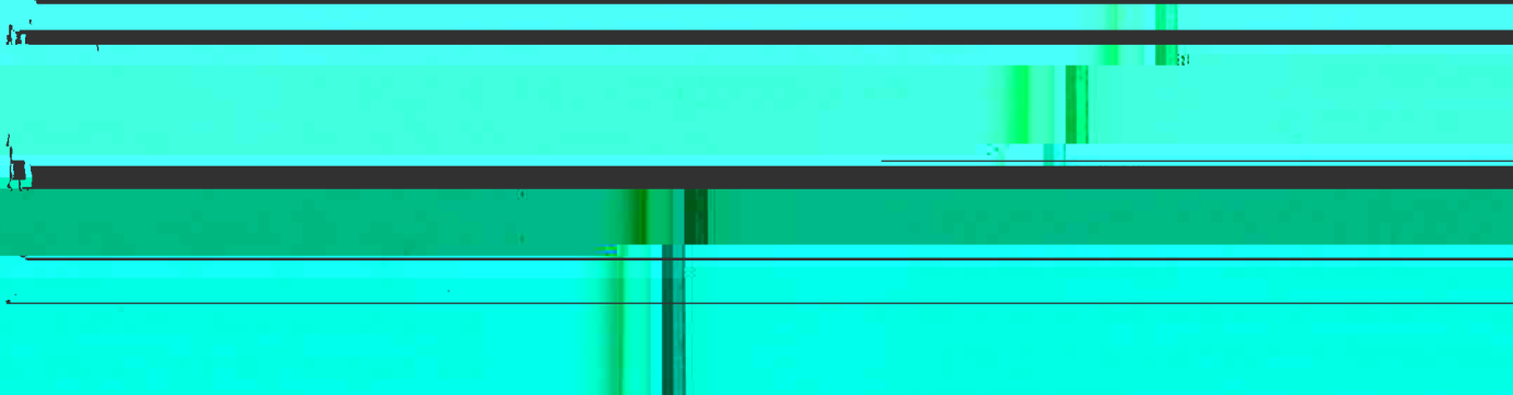
Fig. 1. Electron micrograph of a DNA molecule.
