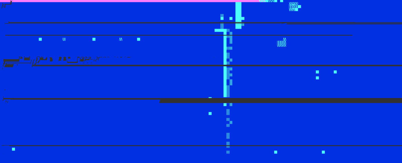
Fig. 2. Electron micrograph of a DNA molecule.
